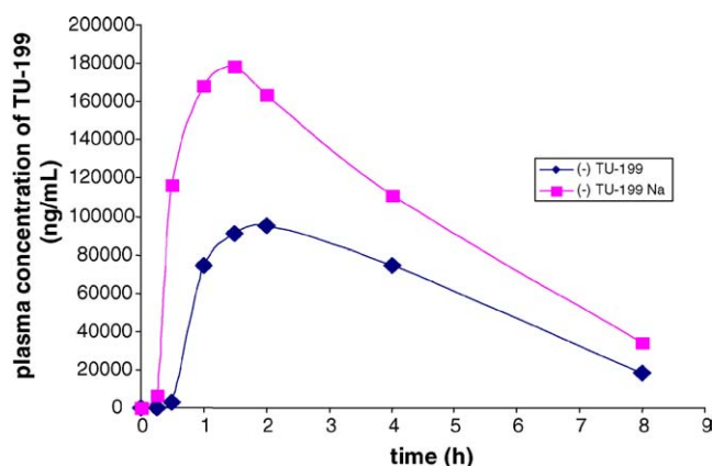
Fig. 9 – The plasma level of tenatoprazole after oral administration. In dogs ( N = 3 ), a dose ( 100 \text{ mg kg}^{-1} ) of (S)-tenatoprazole free form or sodium salt was administrated orally using a capsule contained the compounds as crystallized powder. (–) TU-199 and (–) TU-199 Na represent (S)-tenatoprazole free form and (S)-tenatoprazole sodium salt hydrate form. The results were expressed as mean values.
