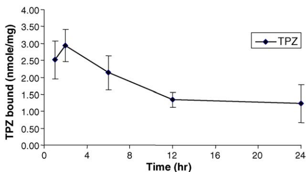
Fig. 5 – Time course of loss of tenatoprazole binding to the H^+,K^+ -ATPase. At timed intervals, crude gastric membranes were collected and ^{14}C -labeling of the H^+,K^+ -ATPase measured as described in experimental procedures using fasted rats. Radioactive ^{14}C -tenatoprazole was administered by IV injection at 0.1 \text{ mCi kg}^{-1} of animal with a dosage of 20 \mu\text{mol kg}^{-1} ( N = 4-6 per each group) through the tail vein. The rats were sacrificed at 1, 2, 6, 12, and 24 h. 'TPZ' represents tenatoprazole-bound gastric membrane. Diamonds (◆) represent average amounts of tenatoprazole binding per milligram of the H^+,K^+ -ATPase in total membrane fraction at each given time point. The results were expressed as mean values \pm S.D. Error bars represent the standard deviation of amounts of tenatoprazole binding ( N = 4-6 for each time point).
