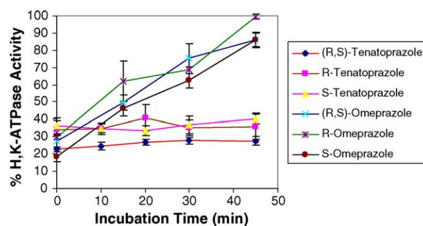
Fig. 7 – Comparison of the time dependent reversal of inhibition of tenatoprazole with omeprazole which is induced by reducing agent. Racemic (R,S)-, S-, and R-omeprazole, racemic (R,S)-, R-, and S-tenatoprazole were compared using ex vivo PPI-inhibited \text{H}^+, \text{K}^+ -ATPase. An aliquot of the PPI-inhibited enzyme in vivo was incubated with 10 mM DTT ( 37^\circ\text{C} ), and its activity assayed at different times after DTT addition. Activity was calculated as the percent of the activity of control ATPase which was not inhibited. The results were expressed as mean values \pm S.D. of at least three experiments.
