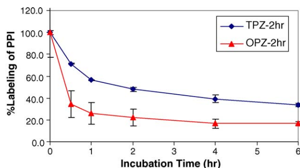
Fig. 6 – Removal of tenatoprazole or omeprazole binding by glutathione. Crude gastric membranes, prepared at 2 h after IV injection of ^{14}\text{C} -labeled drug, were incubated with 10 mM GSH and the amount of labeled \text{H}^+, \text{K}^+ -ATPase was determined as described in the experimental procedure. The percent labeling at the different times of GSH incubation is shown. The points are average of percent PPI binding from five experiments at each given time point and the error bars at each time point represent the standard deviation. TPZ and OPZ represent tenatoprazole and omeprazole, respectively. OPZ-2 h or TPZ-2 h represents the enzyme preparation of 2 h-postdose of omeprazole or tenatoprazole, respectively. The results were expressed as mean values \pm S.D. of five experiments.
